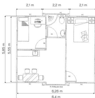
TWO-BEDROOM UNIT HA01
