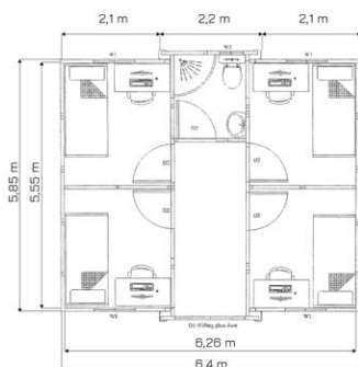
FOUR-BEDROOM UNIT HA04
