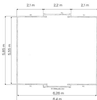
WORK STATION UNIT HA07
