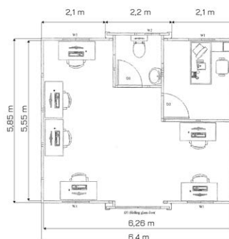
WORK STATION UNIT HA06
