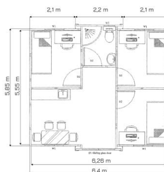
THREE-BEDROOM UNIT HA03
